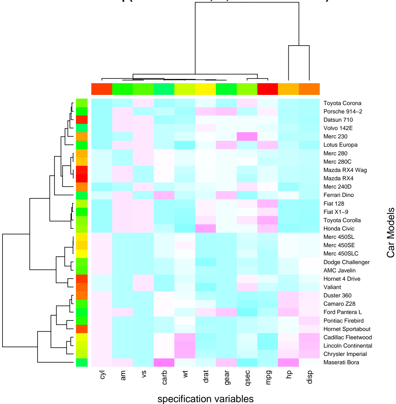
heatmap(<Mtcars data>, ..., scale = "column")
